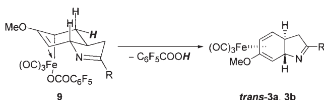
Scheme 1. Plausible mechanism.
